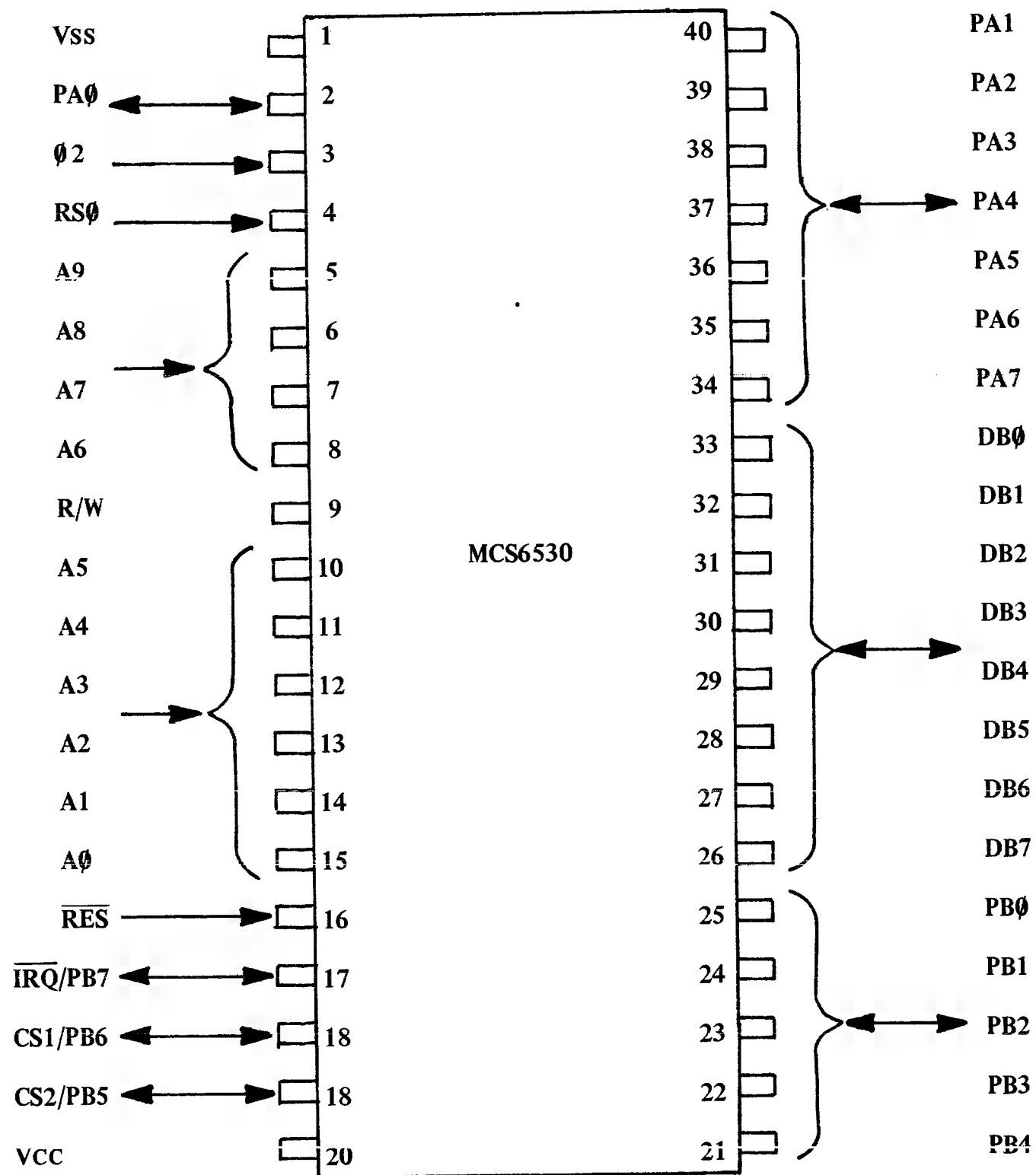
MCS6530 Pinout Designation
